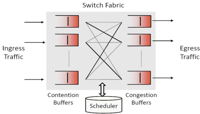
Fig. 1. Buffering in a CIOQ router. Input buffers store packets when there is internal contention. Output buffers store packets when output links are congested.
