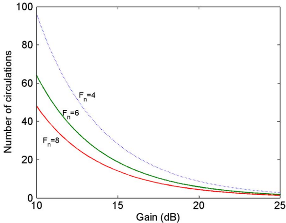
Fig. 12. Maximum number of circulations possible as a function of the loop gain needed in order to maintain an OSNR of 20 dB. Curves are shown for a range of common amplifier noise figures.
