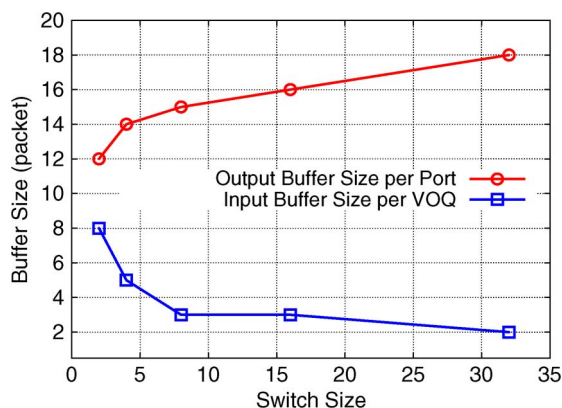
Fig. 15. Minimum required buffer size for 80% utilization versus switch size. The switch has a uniform load distribution, which results in more contention and short-term congestion as the number of ports increases.
