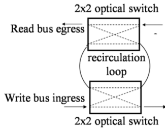
Fig. 9. Physical implementation of speedup and simultaneous read/write.
