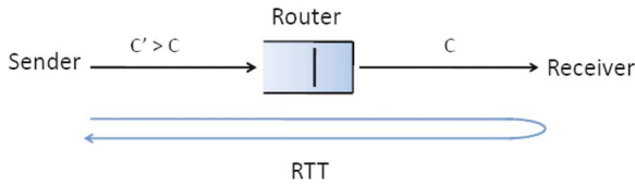
Fig. 2. Single-bottleneck topology. The sender's access link is faster than the receiver's bottleneck link, causing packet accumulation in the router.
