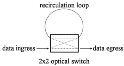
Fig. 8. Schematic of a feedback buffer. A 2 \times 2 switch is combined with a waveguide loop to provide variable delay for an optical signal.
