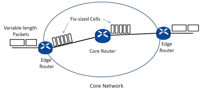
Fig. 13. Core network with fixed-size cells. Edge routers break variable-length packets into small fixed-size cells and reassemble them back into original packets as they depart the core network.
