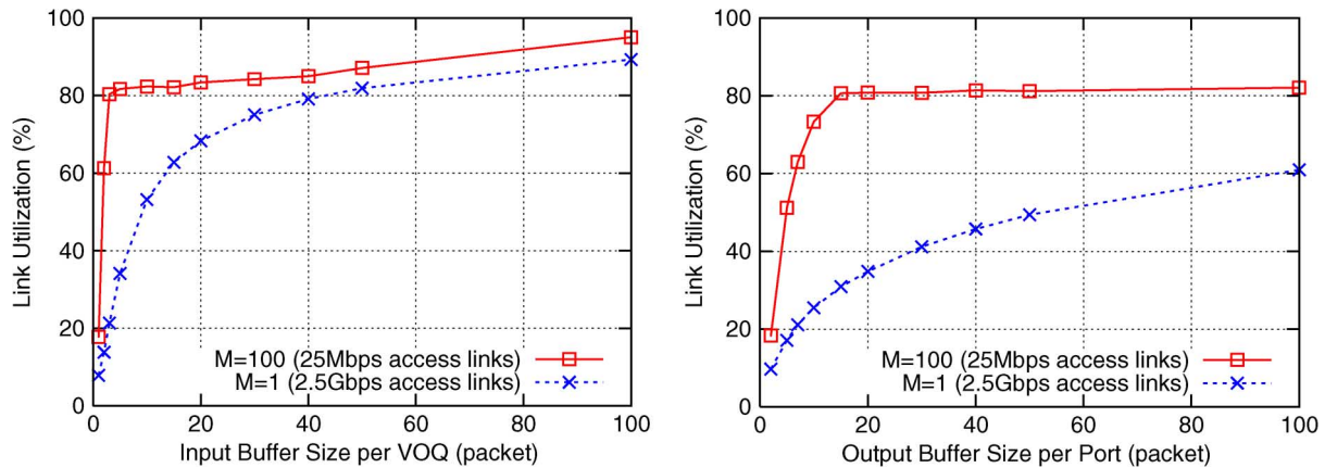
Fig. 6. Link utilization versus input and output buffer sizes. Left: Speedup is 1, and all the queuing takes place at the input. Right: Speedup is 8, and all the queuing takes place at the output. With 25-Mb/s access links, five-packet VOQs and 15-packet output buffers make the utilization above 80%.
