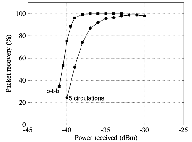
Fig. 11. Packet recovery measurements showing 98% packet recovery for up to five circulations, or 64 ns of storage.
