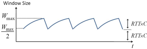
Fig. 3. Window size dynamics of a TCP flow through a bottleneck link. To achieve 100% utilization, the buffer size should be large enough to store RTT \times C packets.
