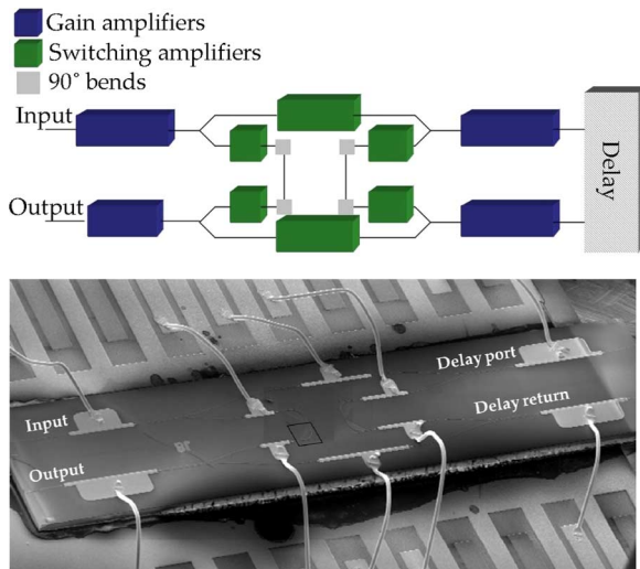
Fig. 10. Schematic and SEM of a fabricated SOA gate matrix switch wire-bonded to an aluminum nitride submount.
