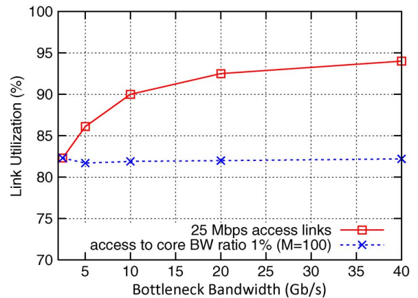
Fig. 7. Link utilization versus bottleneck-link bandwidth. With a fixed access-to-core bandwidth ratio (1%) and a fixed buffer size (20 packets), increasing the bottleneck-link bandwidth does not change the utilization.
