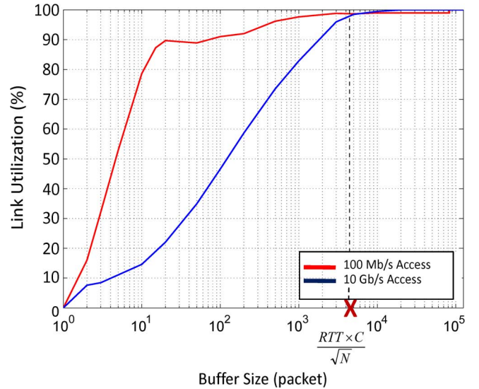
Fig. 4. Link utilization versus buffer size. With 800 flows on the link, close to 100% utilization is achieved if the buffer size is RTT \times C / \sqrt{N} . If flows come from slower access links, a tiny buffer size of 10 packets suffices for 80% utilization.
