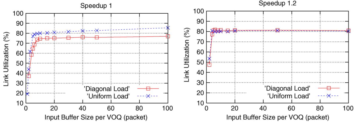
Fig. 14. Link utilization versus buffer size with iSLIP. Left: speedup = 1. Right: speedup = 1.2.
