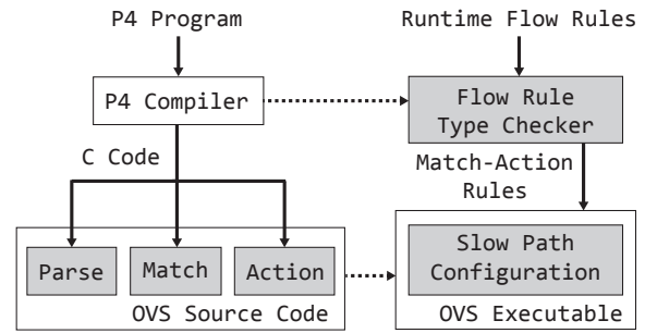
Figure 3: The P4-to-OVS Compiler in PISCES.
