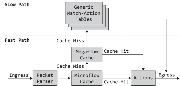
Figure 2: OVS forwarding model.
