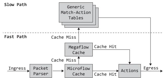
Figure 2: OVS forwarding model.
