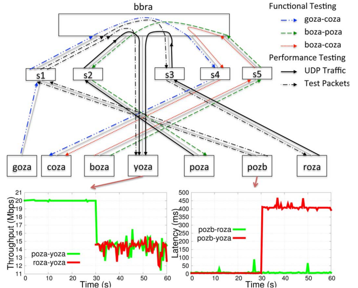
Fig. 9. Portion of the Stanford backbone network showing the test packets used for functional and performance testing examples in Section VII-C.
