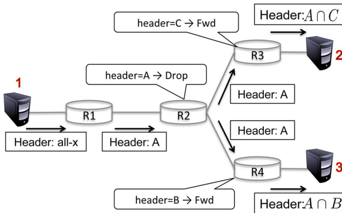
Fig. 7. Generate packets to test drop rules: “flip” the rule to a broadcast rule in the analysis.
