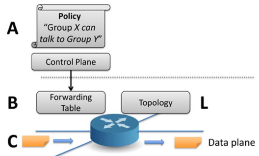
Fig. 1. Static versus dynamic checking: A policy is compiled to forwarding state, which is then executed by the forwarding plane. Static checking (e.g., [16]) confirms that A = B . Dynamic checking (e.g., ATPG in this paper) confirms that the topology is meeting liveness properties ( L ) and that B = C .
