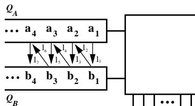
Figure 12: 2 \times N multicast crossbar switch. The links show the order in which cells are released.
