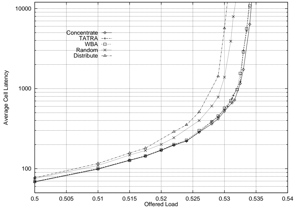
Figure 6: Graph of average cell latency (in number of cell times) as a function of offered load for a 2 \times 8 switch (Correlated arrivals with an average fanout of four).
