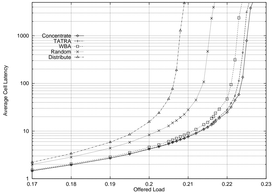
Figure 7: Graph of average cell latency (in number of cell times) as a function of offered load for an 8 \times 8 switch (Uncorrelated arrivals with an average fanout of four). Note that the total load on the switch is four times the offered load at the inputs.
