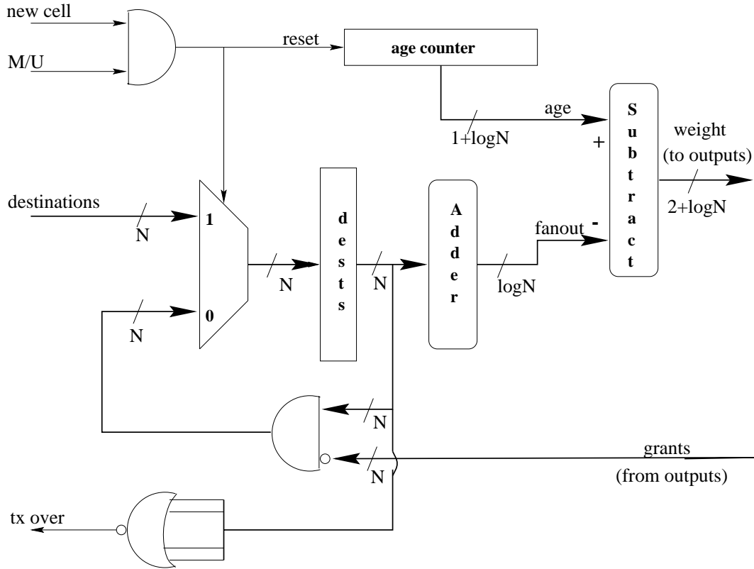
Figure 9: The hardware required in WBA for computation of weight at each input. The age counter is reset when a new multicast cell comes to HOL, and is incremented every cell time thereafter. The bits corresponding to the outputs, which grant to this input, are selectively reset in every cell time until the entire destination vector (the register dests ) becomes zero. At this point, the input port is signalled that the transmission of the cell is over, so a new cell can come to HOL. Since the maximum age of a cell at HOL is 2N - 1 for an N \times N switch, the age counter needs to be 1 + \log(N) bits wide. Subtracting the fanout (which spans from 1 to N ) from the age makes the total range of weights to be 3N - 1 , which can be represented by using 2 + \log(N) bits.
