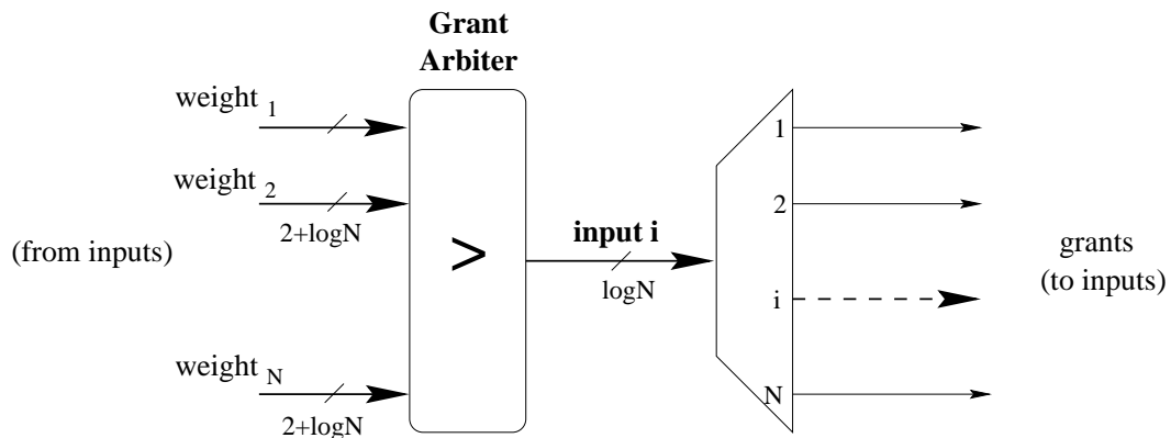
Figure 10: The hardware required in WBA for determining the input to grant to, at each output. The input requesting with the highest weight is selected.
