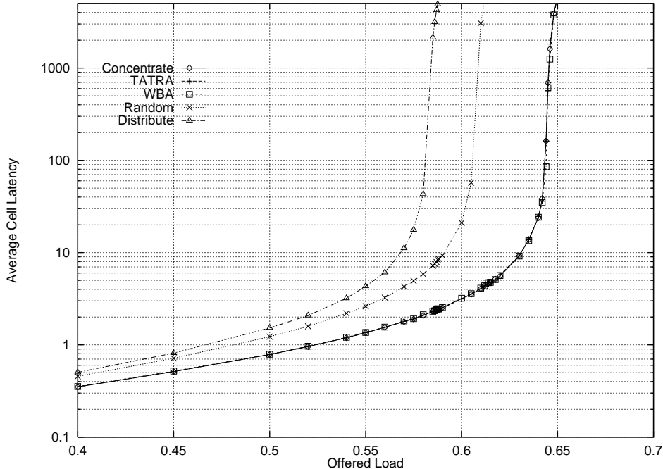
Figure 5: Graph of average cell latency (in number of cell times) as a function of offered load for a 2 \times 8 switch (Uncorrelated arrivals with an average fanout of four).
