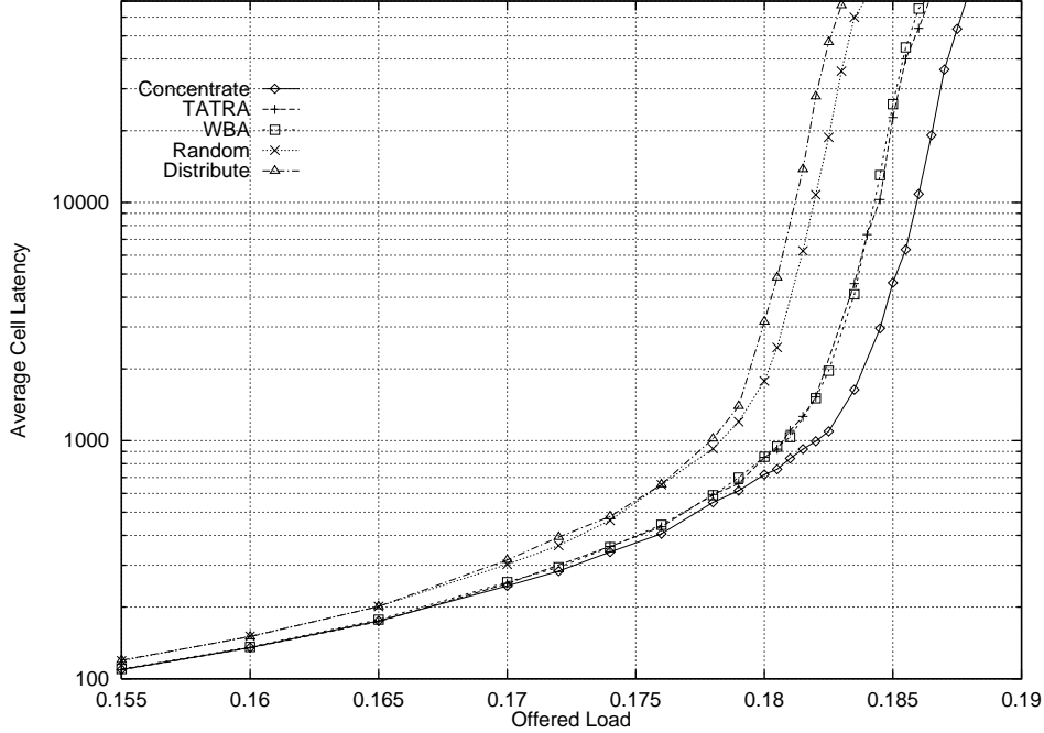
Figure 8: Graph of average cell latency (in number of cell times) as a function of offered load for an 8 \times 8 switch (Correlated arrivals with an average fanout of four).
