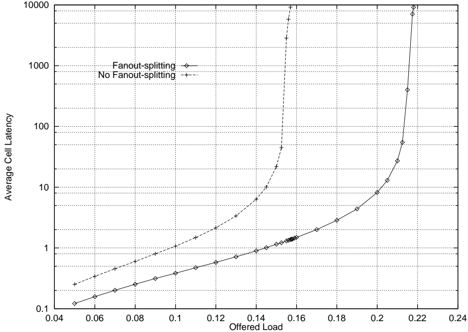
Figure 2: Graph of average cell latency (in number of cell times) as a function of offered load for an 8 \times 8 switch (with uniform input traffic and average fanout of four). The graph compares Random scheduling policy with and without fanout-splitting.
