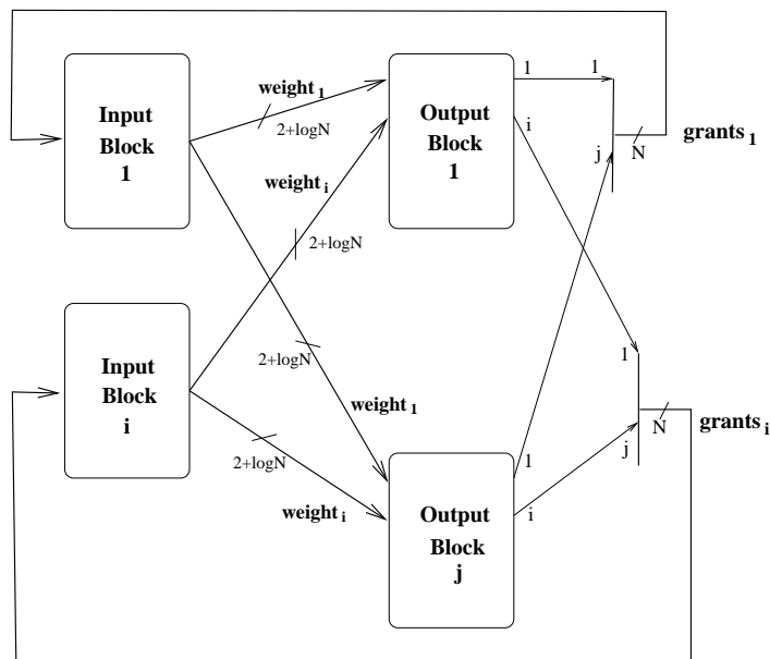
Figure 11: Connecting N input blocks and N output blocks to form an N \times N WBA scheduler.
