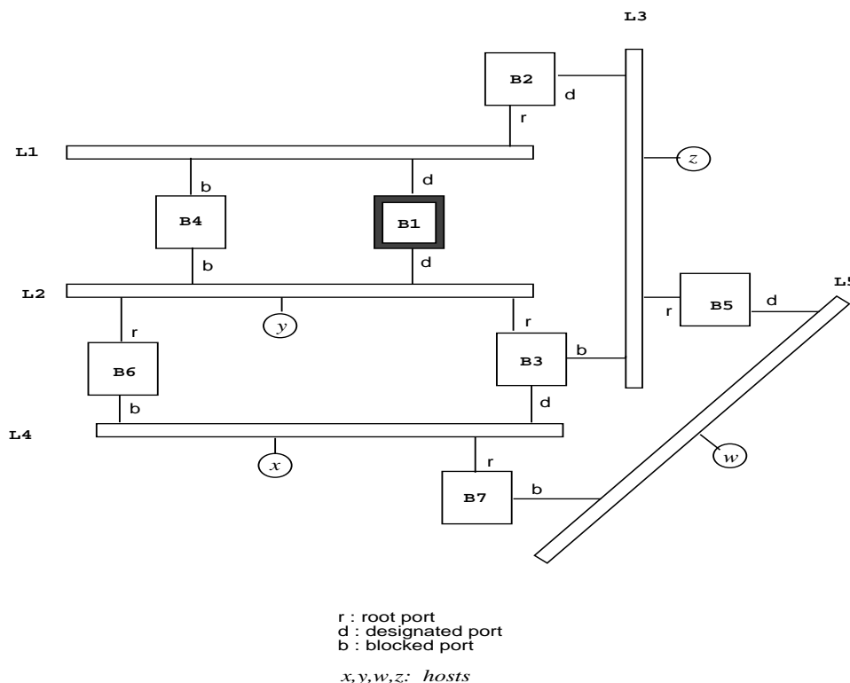
Figure 8: Sample Network after Spanning Tree Algorithm converges
